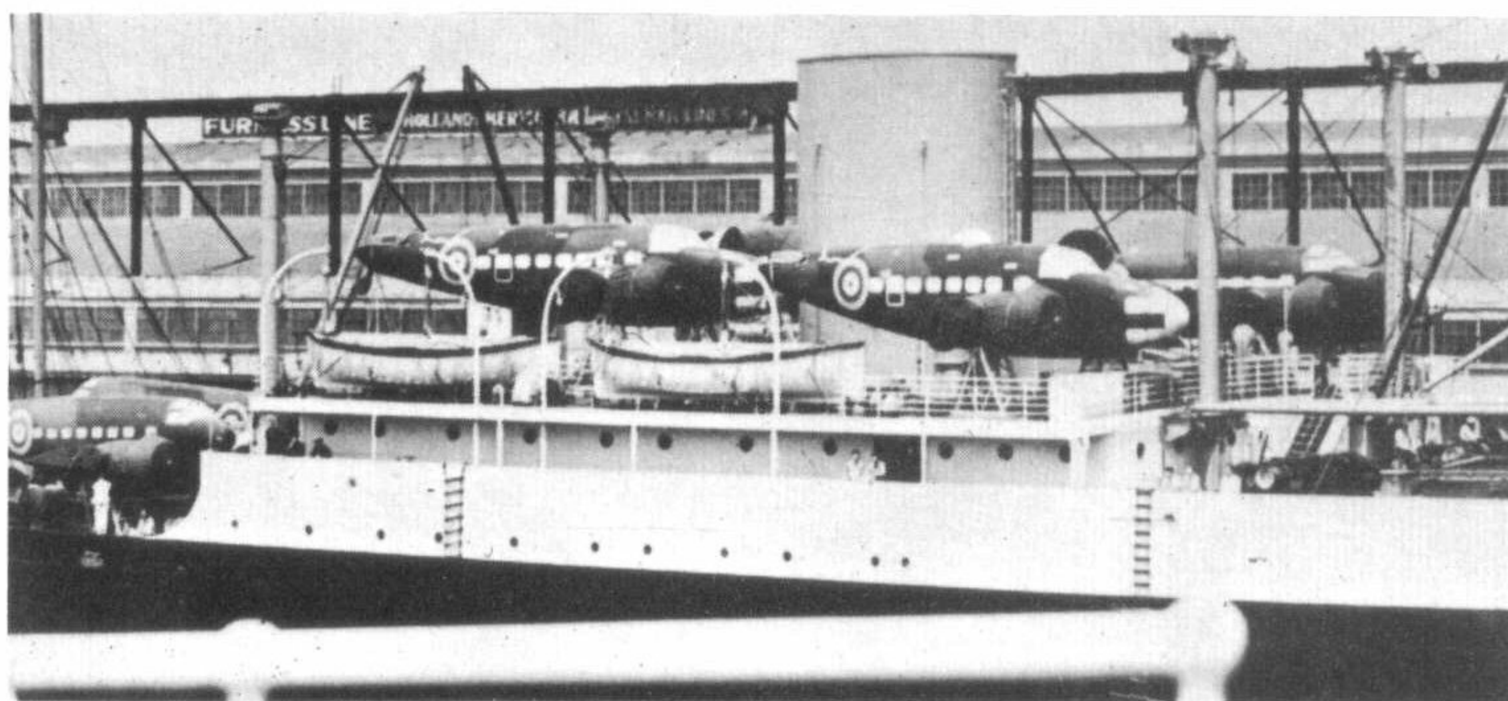
One of the very few photographs showing the method of shipping Hudson Mk Is from Los Angeles to Liverpool. Here, the British motorship m.s. Lockhaven, about to depart in late May 1939, has no fewer than six as deck cargo.
